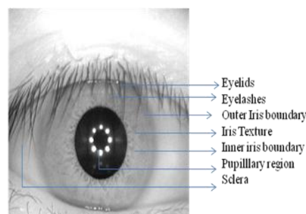
Figure 1: Iris image
