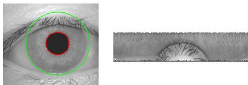
Figure 3 Iris normalization
