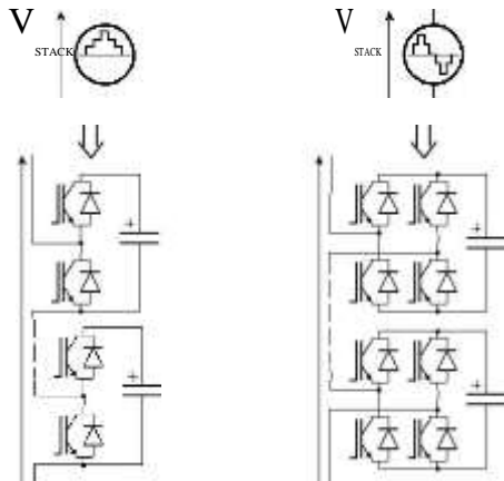
Fig. 1. Electrical schematic of half-bridge cells (left) and H-bridge cells (right).
