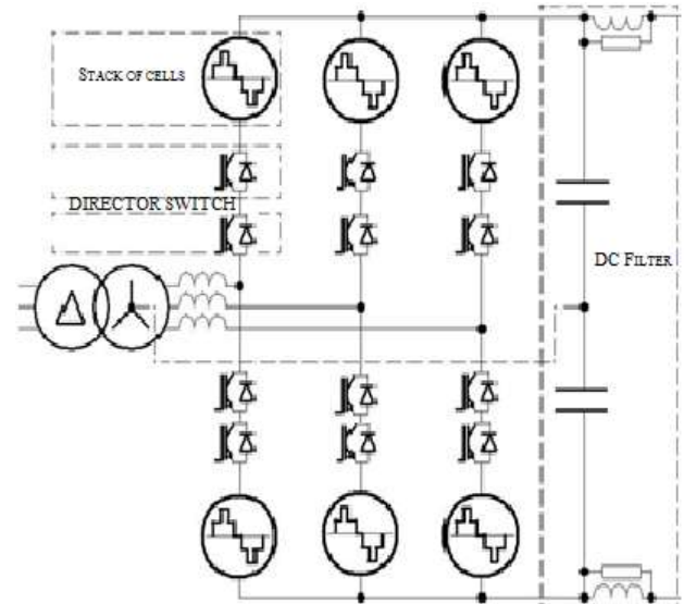
Fig. 2 Schematic of the Alternate Arm Converter, with the optional middle-point connection shown in dashed line.
