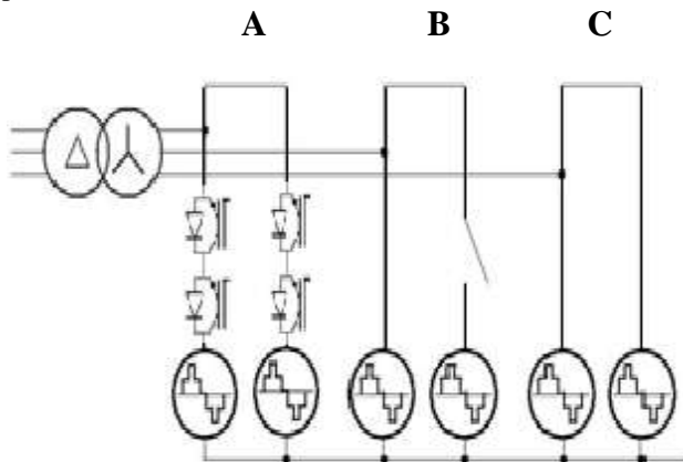
Fig. 4. STATCOM modes of the AAC during a DC-side fault: alternate arms (mode A), single working arm (mode B), dual working arms (mode C)
