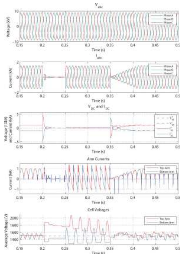
Fig. 6. Simulation results of a 20-MW AAC model running in rectifier mode when a dc-side fault occurs between 0.20 and 0.35 s.
