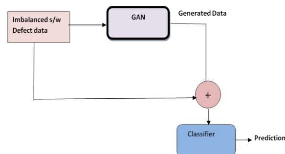
Figure 2: Flow Diagram for Data Augmentation using GANs
